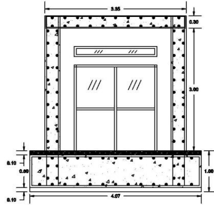
SECTION X-X
