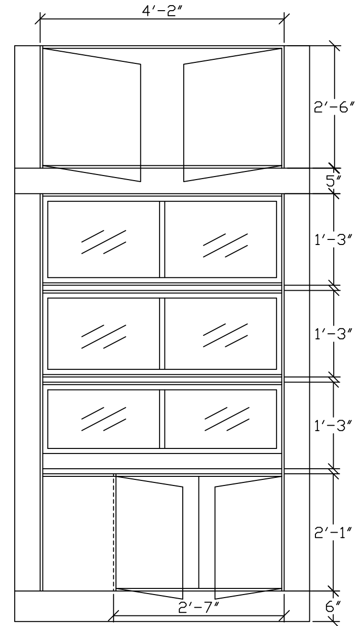
STORAGE UNIT
