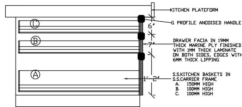
SECTION QQ
