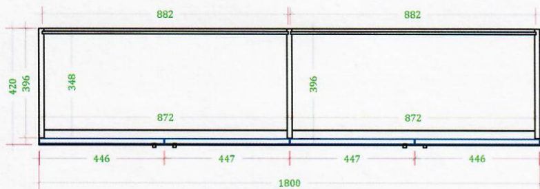
SECTIONAL PLAN AT -AA'
