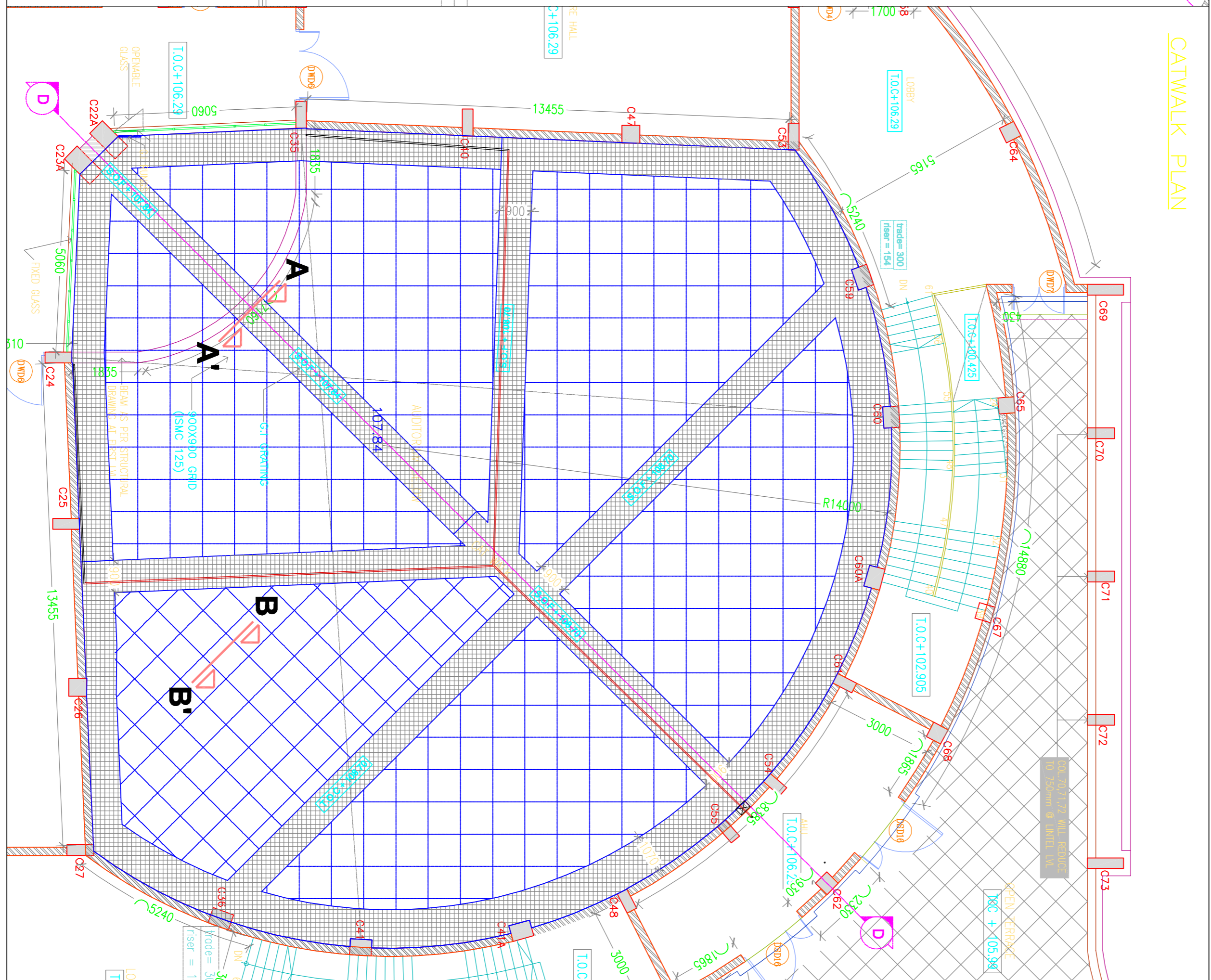
BASEMENT FALSE CEILING LAYOUT
